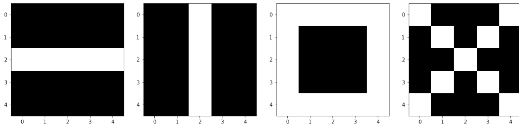
Figure 3: 5 \times 5 grids of patterns stored in the memory model
